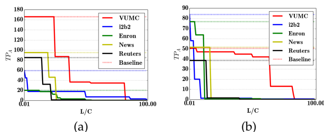
Fig. 3. The number of residual true positive instances TP_A , which is equivalently the identified instances for an attacker with a small budget after running GS for the i2b2, VUMC, Enron, Newsgroup, and Reuters datasets. We evaluate (a) GS using CRF; (b) GS using the best classifier from {CRF, SVM, AdaBoost, Ensemble}. The dashed lines correspond to the baseline application of the best classifier from this collection.
