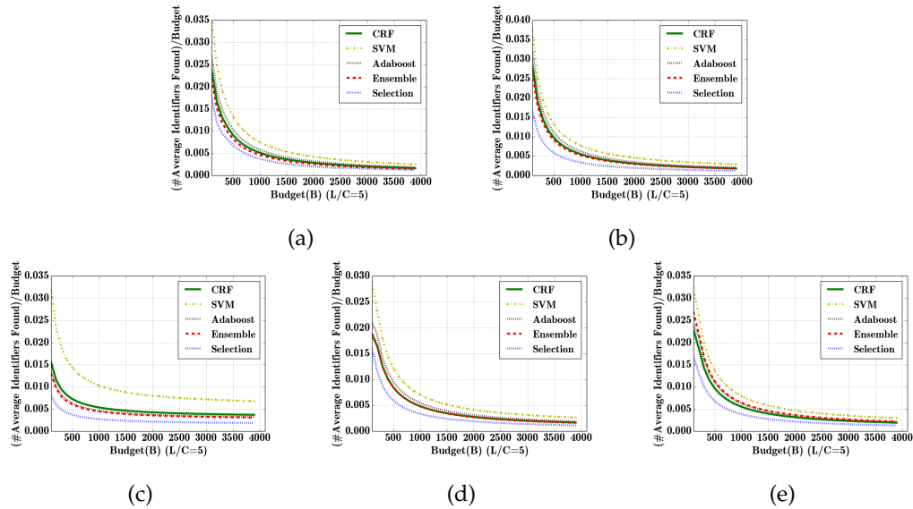
Fig. 6. The ratio of the average number of sensitive identifiers found by the attacker and the adversarial budget, while the publisher applies classifiers CRF, SVM, AdaBoost, Ensemble, and Selection which allows the publisher to choose a learner with highest accuracy from {CRF, SVM, AdaBoost, Ensemble} for GS (L/C=5). (a) i2b2, (b) VUMC, (c) Enron, (d) Newsgroup, and (e) Reuters datasets.
